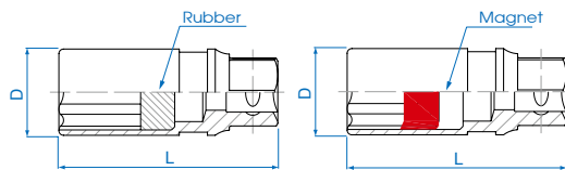
463516R - Thin walled design
