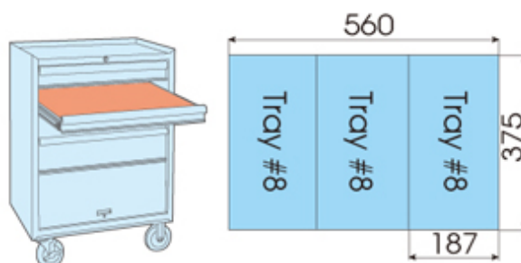
Drawer B3(579x380)
